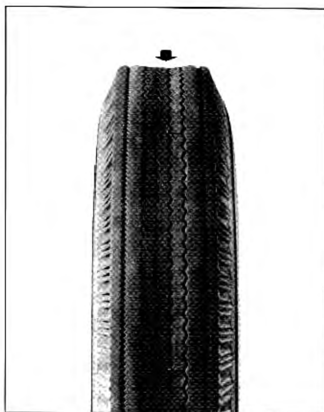
Fig. 10-4 Wear from Overinflation
