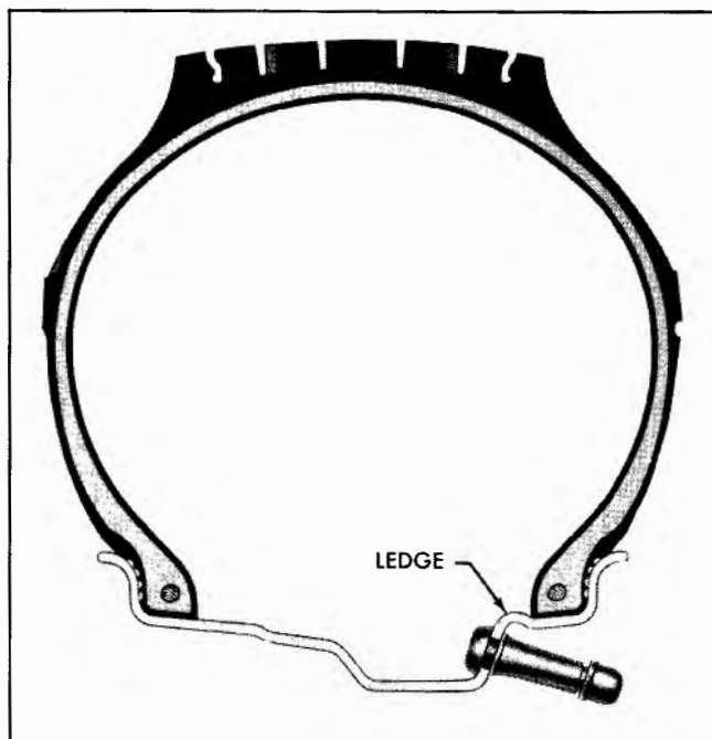
Fig. 10-1 Cross Section of Typical Tubeless Tire
